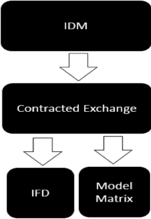
Figure 3.11: IDM content
