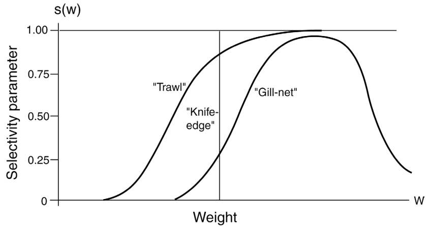
Figure 8.5. Selectivity curves for three types of fishing gear.
