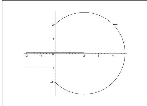
Figure 1: A possible curve \mathcal{K} from -2i to 2i without intersecting the lines L_1 and L_2 .
