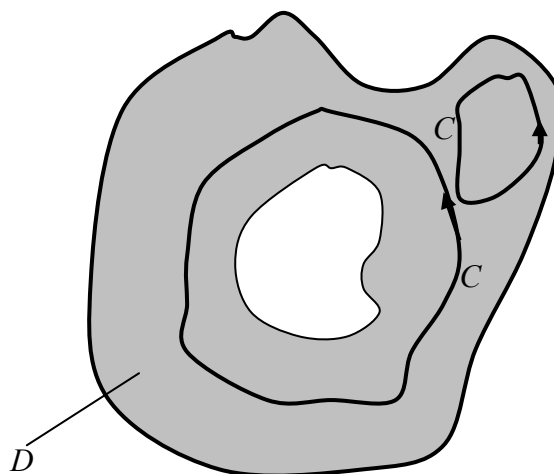
multiply connected
