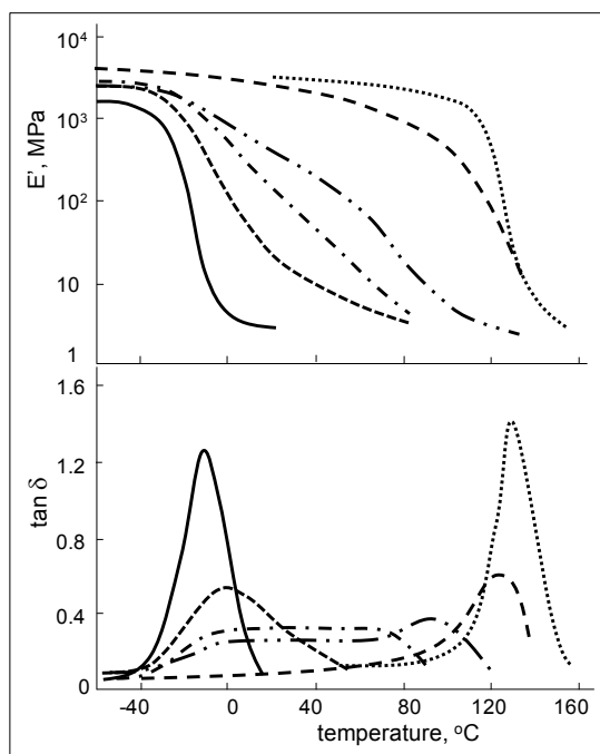
Figure 7.25 E' and \tan \delta vs. temperature for PU/PMMA compositions by weight of (—) 100/0; (---) 80/20; (- · - ·) 70/30; (- · · ·) 50/50; (- - - -) 20/80 and (.....) 0/100 (source: Akay & Rollins 1993)
