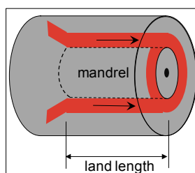
Figure 3.23 Description of a land length for a die and mandrel or pin used for a tubular product
