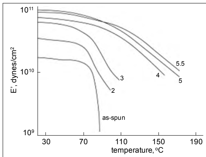
Figure 7.20 Storage modulus ( E' ) vs. temperature for PET fibres drawn at various draw ratios. The draw ratios are indicated on the curves (note that 1 dyne/cm 2 = 0.1 Pa) (source: Miller 1984)
