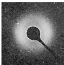
Figure 4.8 Generation of a SAXS pattern from lamellae
