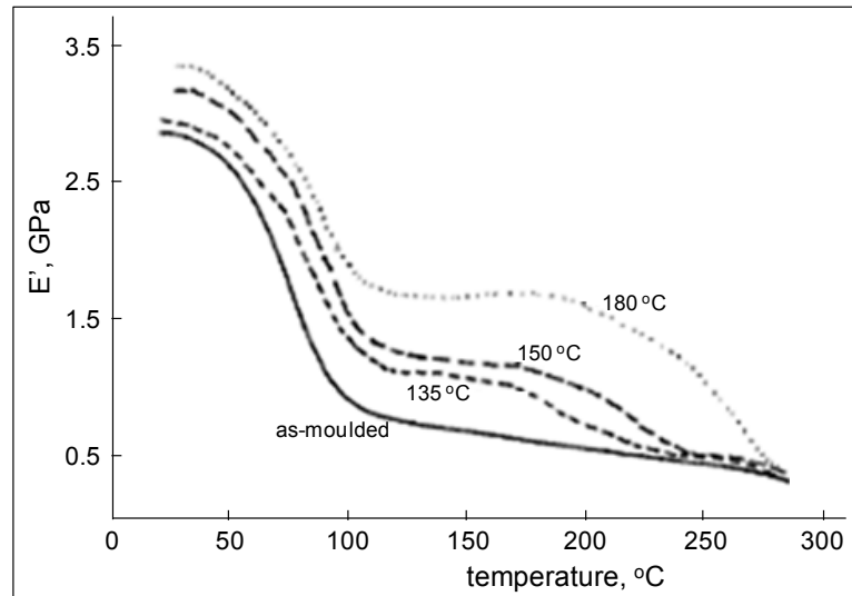
Figure 7.18 Storage modulus ( E' ) vs. temperature for Nylon 66: as-moulded and heat treated at 135, 150 and 180 °C (source: Sepe 1997, p29)
