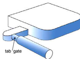
Figure 3.11 Tab gate (source: http://www.dsm.com/en_US/html/dep/gatetype.htm )
