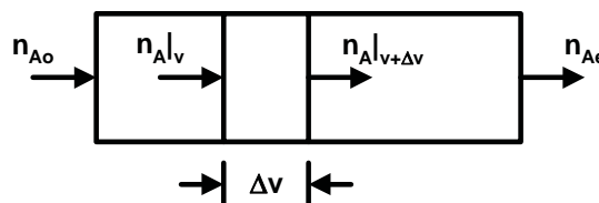
Figure 1.3 The mass balance of a (“plug”) volume element in a tubular reactor
