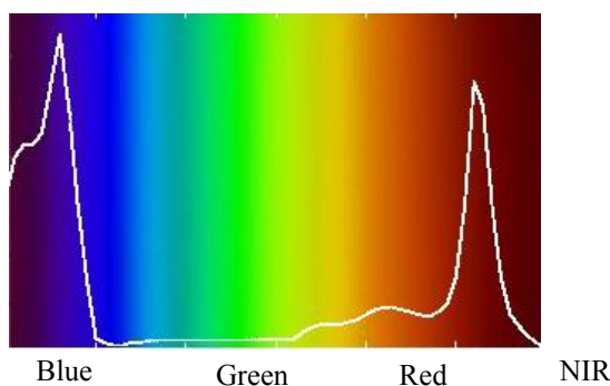
Figure 4.5 Absorption spectrum of a typical plant
