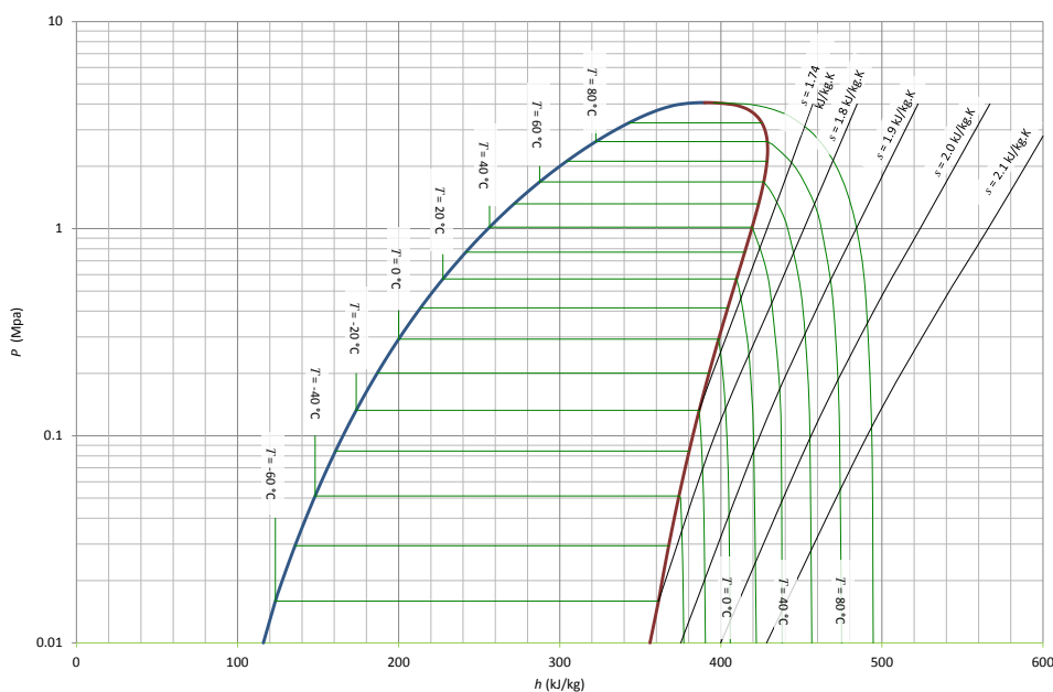
Figure 2.6: Pressure-enthalpy diagram for Refrigerants R-134a
