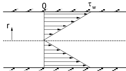
Figure 4-6: Shear stress distribution in a liquid flowing laminarily through a pipe.
