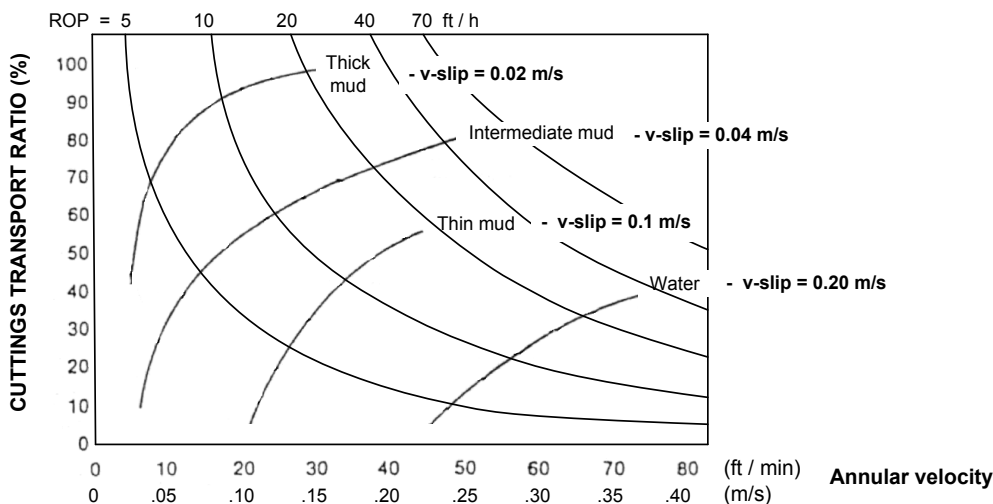
Figure 6-5: Annular velocity in a 5 * 1 1/4 " annulus to keep cuttings concentration above 4 vol %.
