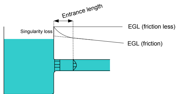
Figure 4-2: After entrance effects flow reaches a stationary flow profile.
