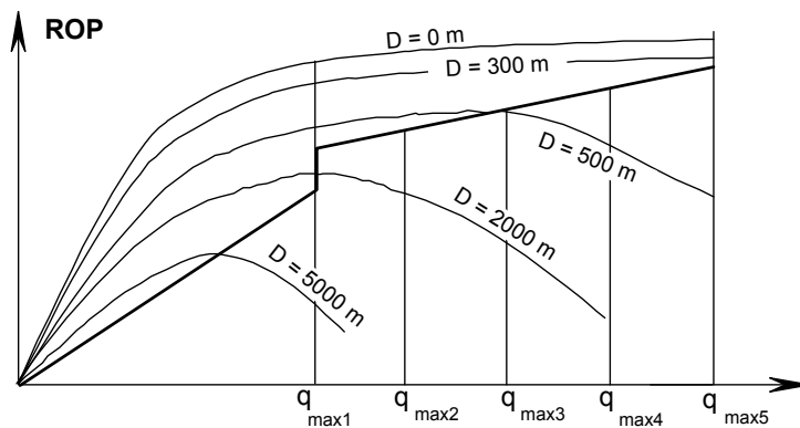
Figure 5-5: ROP (eqn. (5.10) in range I and eqn. (5.17) in range II) vs. pump rate and depth.
