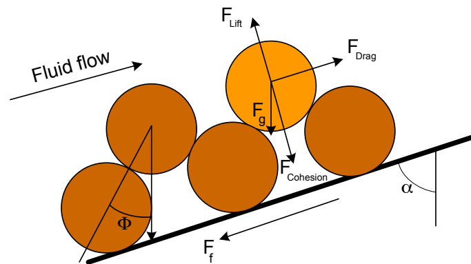
Figure 6-7: Forces acting on particle at an active erosion site of a cuttings bed. \phi is the angle of repose.
