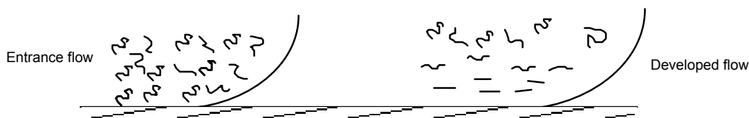
Figure 3-14: Polymers as drag reducers; low viscosity develops at the wall.
