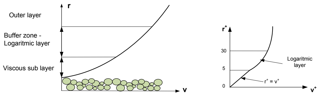
Figure 6-8: Near-bed velocity profile. Increased roughness will lead to increased drag due to increased local velocity. In the viscous sub layer dv^+/dr^+ is assumed to be 1. dr^+ = r/R , v^+ = v/v_{max} .
