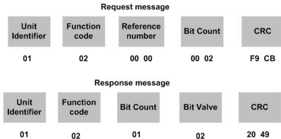
Figure 5.9 Example: FC02-reading input discretres
