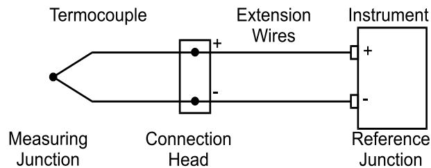
Figure 11.6 Typical thermocouple and extension leads
